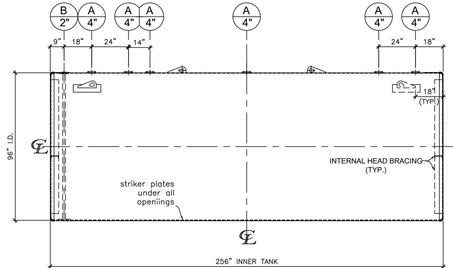
FRONT VIEW
