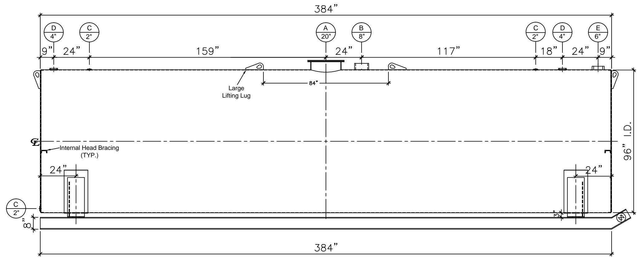
FRONT VIEW
