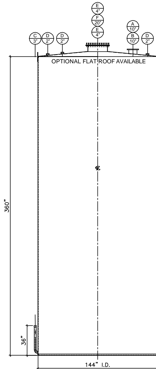
FRONT VIEW
