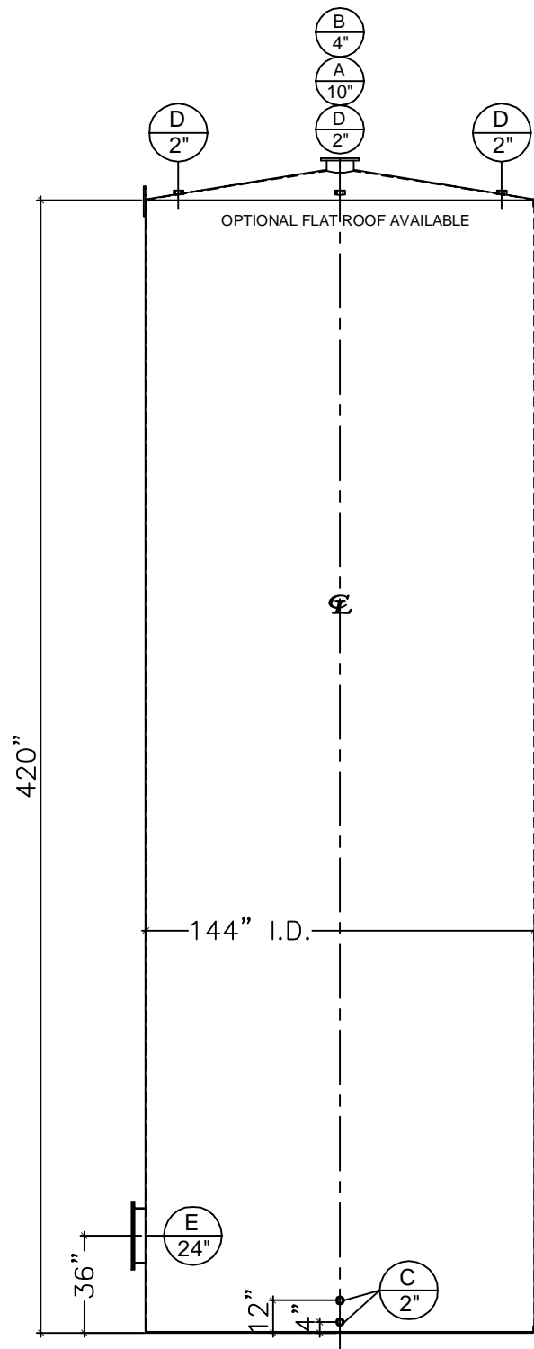
FRONT VIEW
