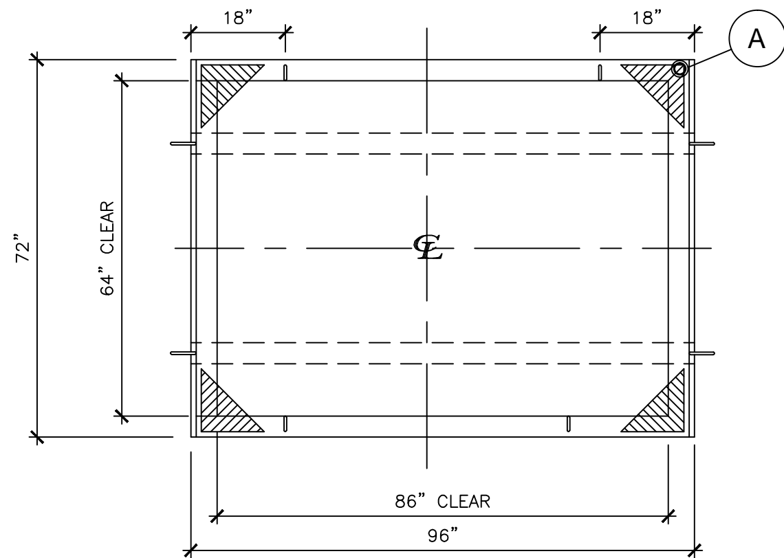
PLAN VIEW
