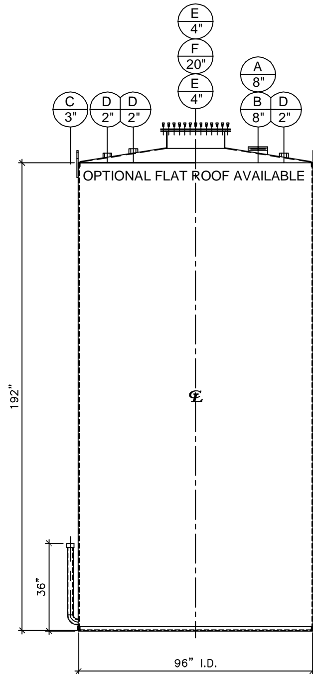
FRONT VIEW
