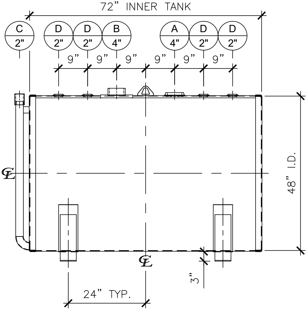
FRONT VIEW
