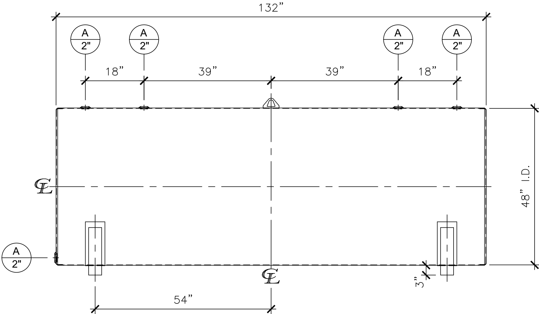
FRONT VIEW
