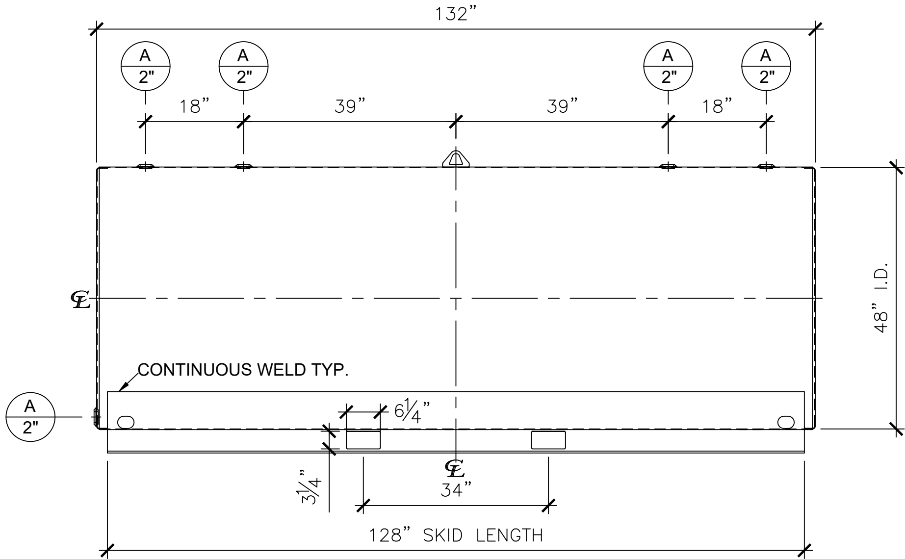
FRONT VIEW
