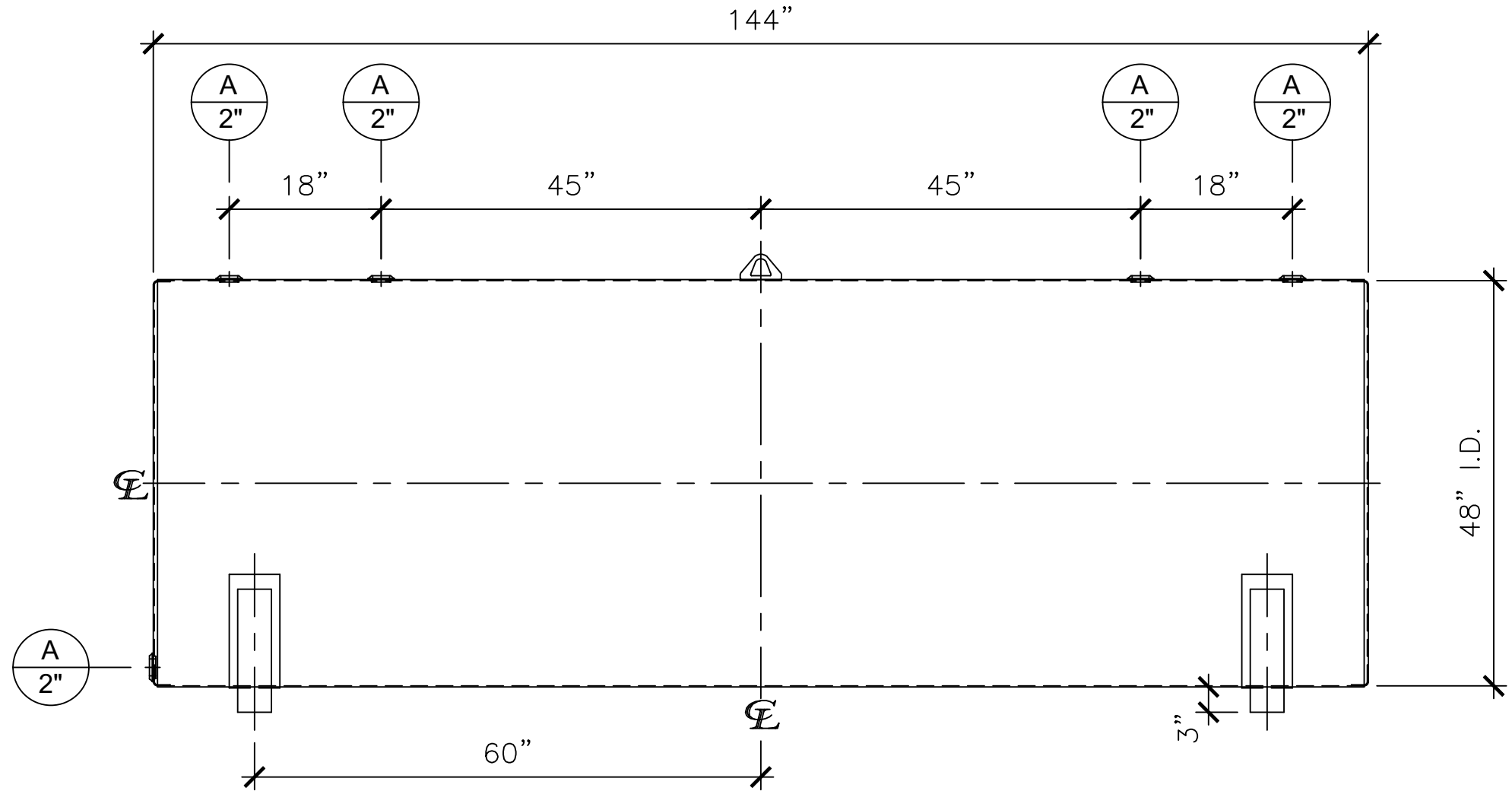
FRONT VIEW
