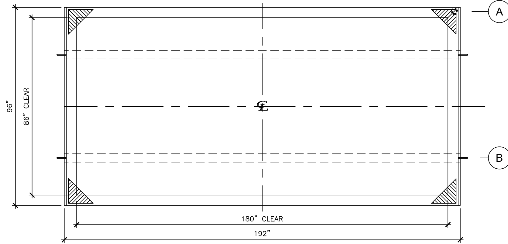
PLAN VIEW
