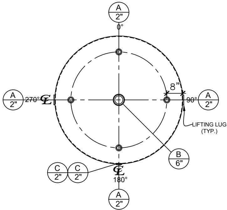
PLAN VIEW
