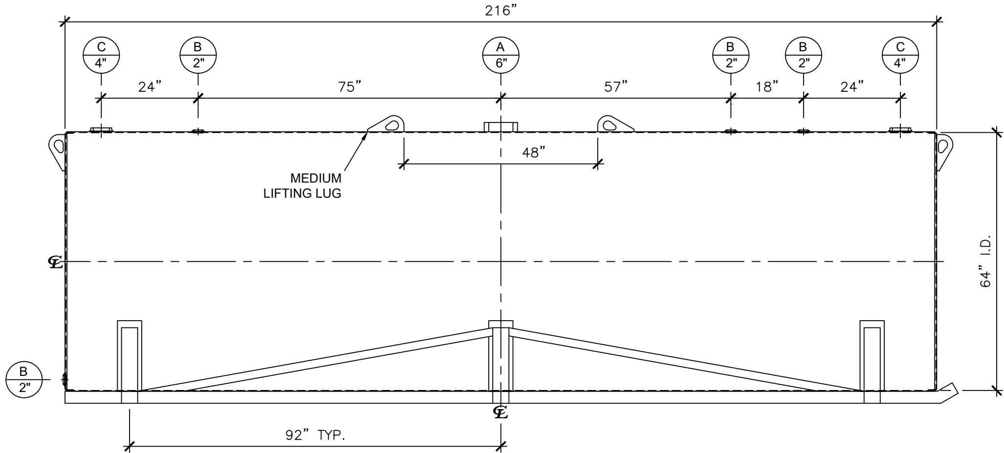
FRONT VIEW
