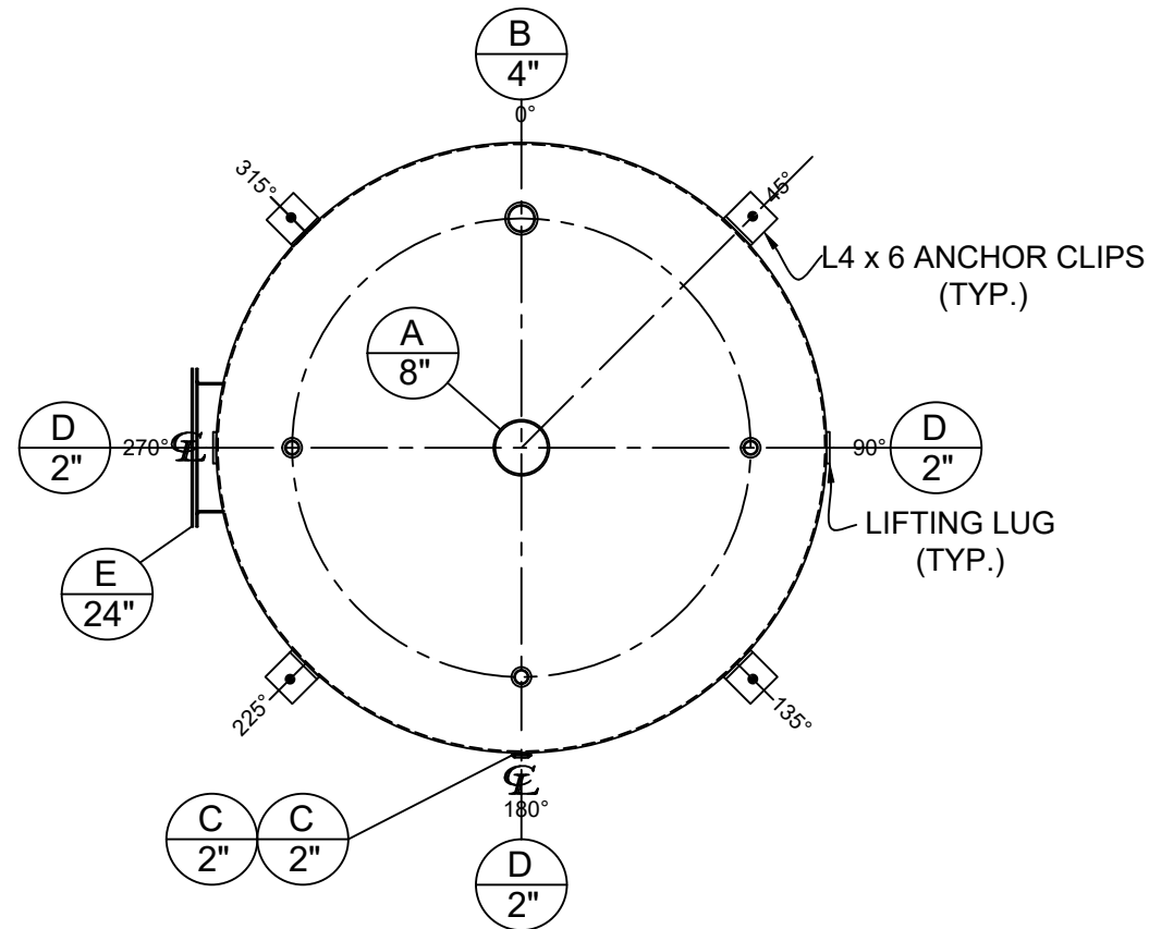
PLAN VIEW
