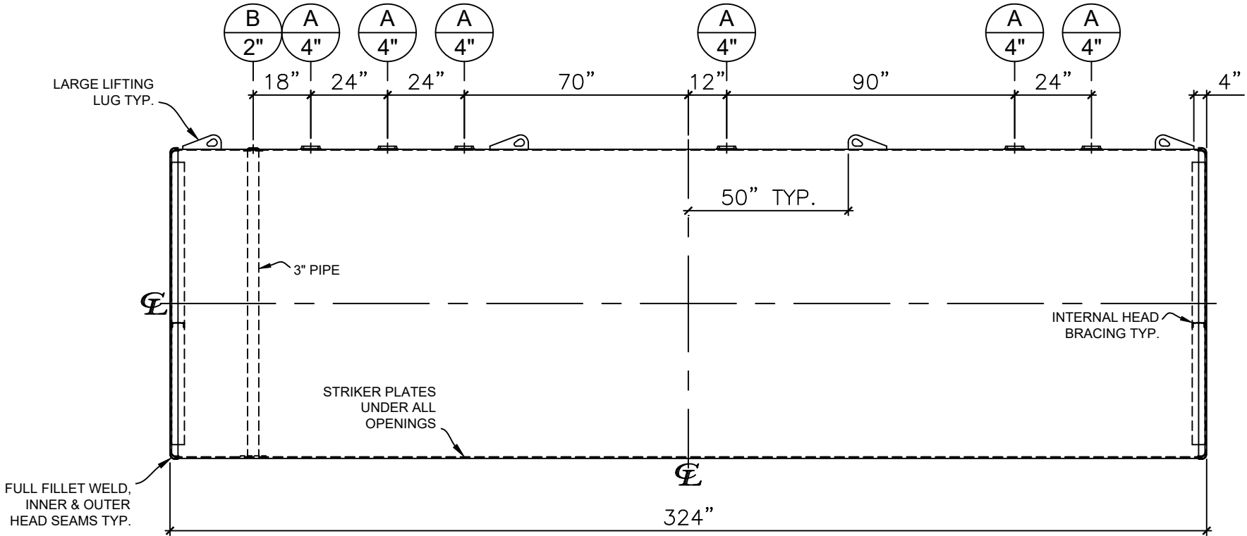
FRONT VIEW
