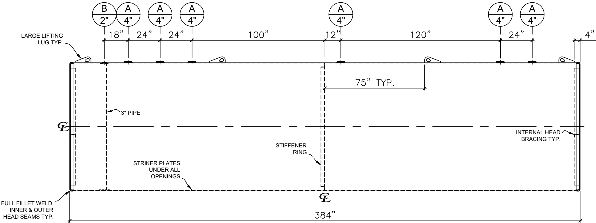
FRONT VIEW
