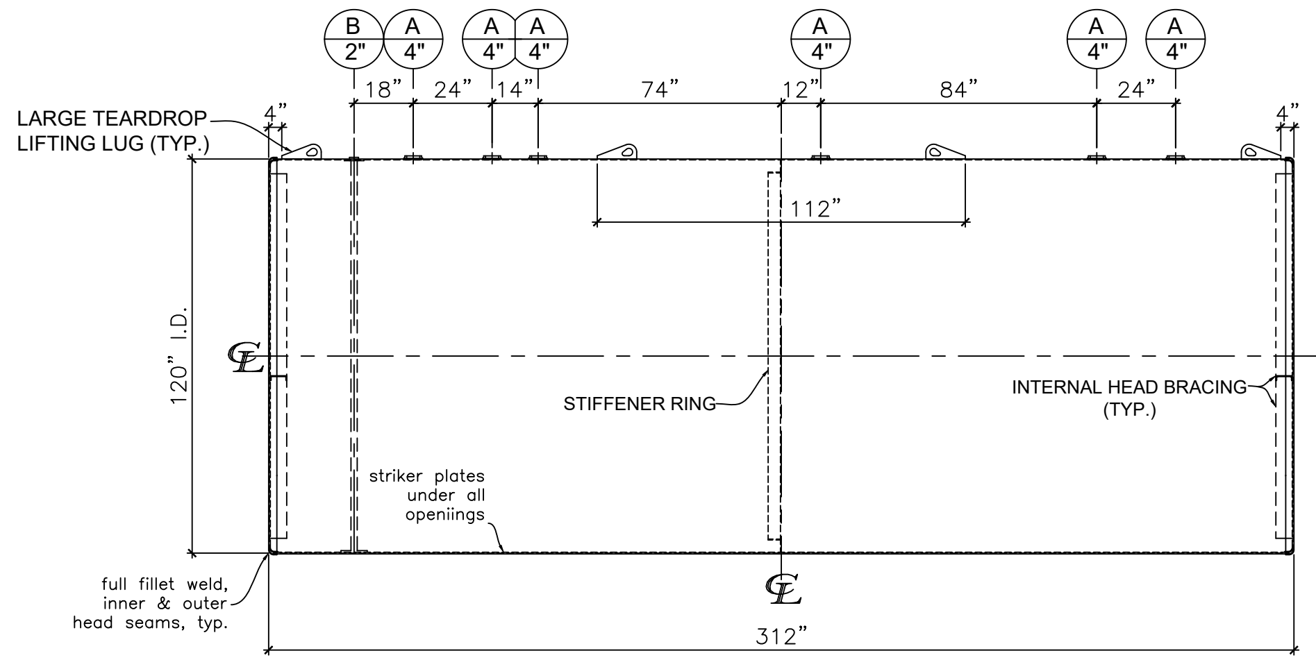
FRONT VIEW
