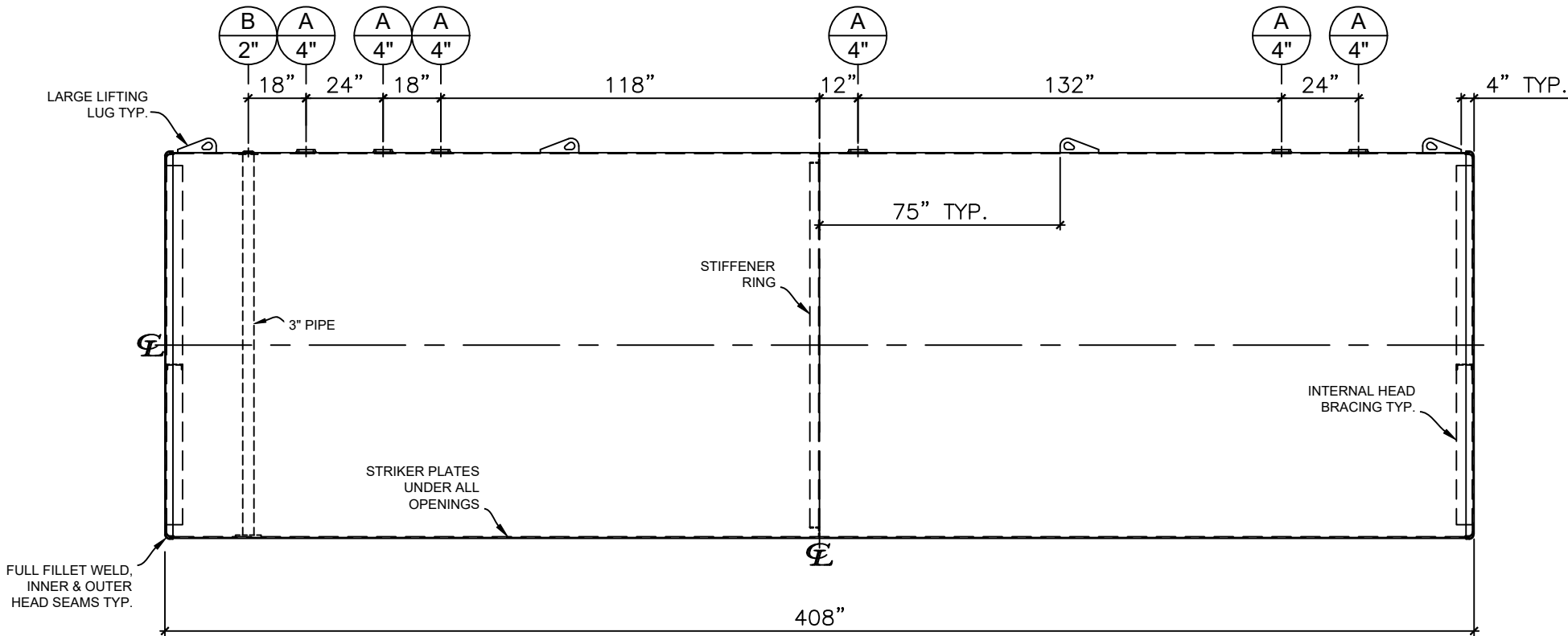
FRONT VIEW
