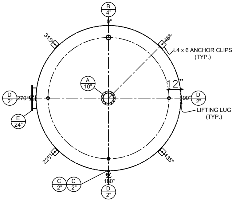
PLAN VIEW
